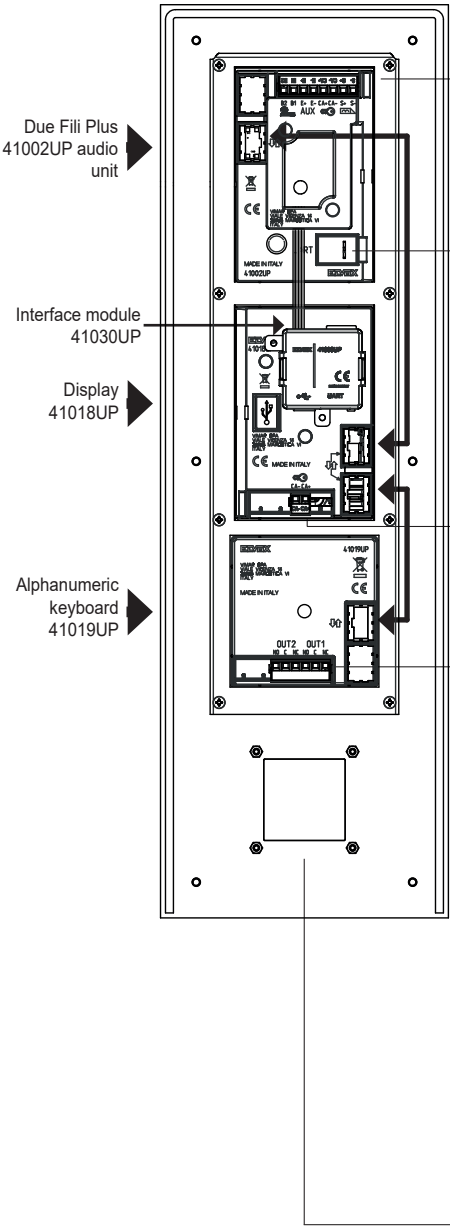
40424 audio entrance panel rear view
