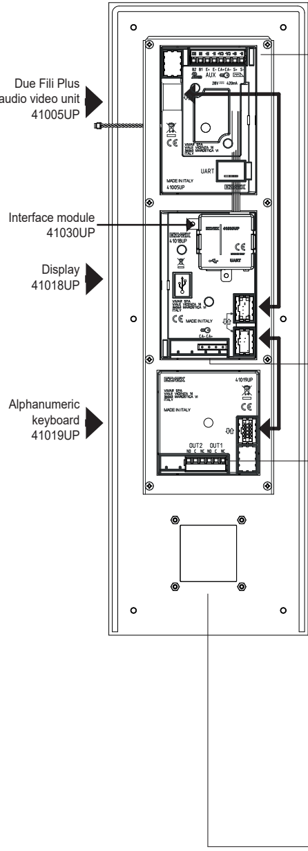
40404 audio/video entrance panel rear view
