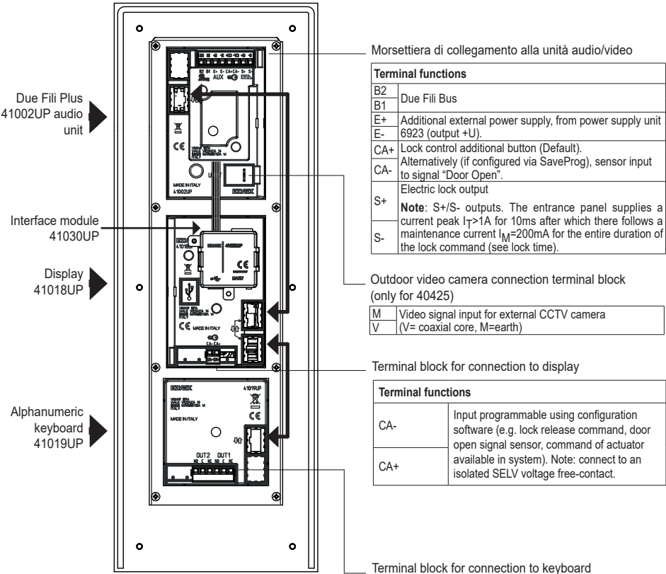
40425 audio entrance panel rear view
